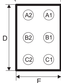
Chip Scale Package (Bottom View)
